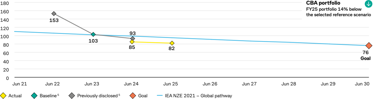
Aviation emissions intensity 4 gCO 2 /revenue passenger km
